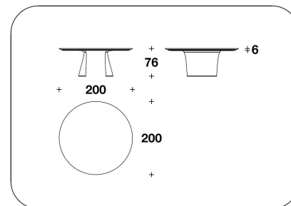
BTV (30EE) - BTV (30EP) ROUND : TAVOLO / TABLE Ø 200x76H. - THK.6cm Ø 78 2/3x30H. - THK.2 6/16"
