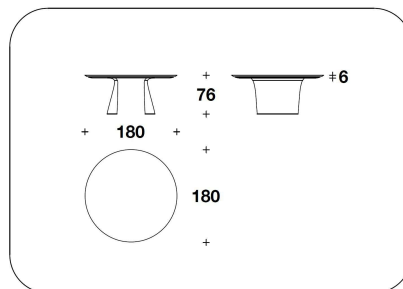
BTV (32ME) - BTV (32MP) ROUND MARBLE : TAVOLO / TABLE Ø 180x76H. - THK.6cm Ø 71x30H. - THK.2 6/16"
