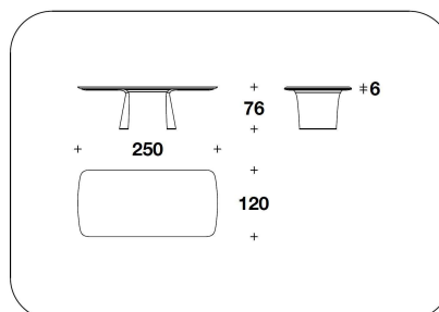
BTV (31EE) - BTV (31EP) RECTANGULAR : TAVOLO / TABLE 250x120x76H. - THK.6cm 98 1/3x47 1/3x30H. - THK.2 6/16"
