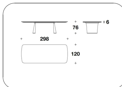
BTV (29ME) - BTV (29MP) RECTANGULAR MARBLE : TAVOLO / TABLE 298x120x76H. - THK.6cm 117 1/3x47 1/3x30H. - THK.2 6/16"
