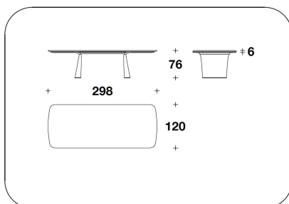
BTV (29EE) - BTV (29EP) RECTANGULAR : TAVOLO / TABLE 298x120x76H. - THK.6cm 117 1/3x47 1/3x30H. - THK.2 6/16"
