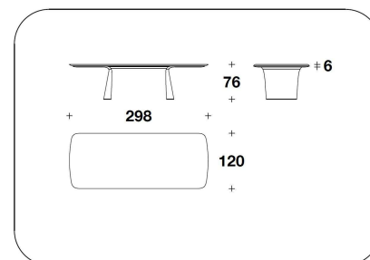
BTV (31ME) - BTV (31MP) RECTANGULAR MARBLE : TAVOLO / TABLE 250x120x76H. - THK.6cm 98 1/3x47 1/3x30H. - THK.2 6/16"
