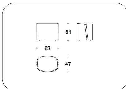
CTB (25E) - CTB (25P) SIDE TABLE 63x47x51H.cm 24 2/3x18 2/4x20H."
