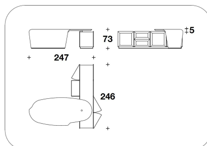
BTV (19MP) - BTV (19ME) - BTV (19CP) - BTV (19CE) OPTIONAL 1 - OPTIONAL 2 x BTV (19) L.240x108x73H. - 247x246x73H.cm L.94 1/3x42 2/3x28 2/3H. - 97 1/3x97x28 2/3H."
