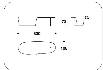
BTV (21E) SYCAMORE - BURR WALNUT : SCRIVANIA DX O SX / RIGHT OR LEFT WRITING-DESK L.300x108x73H. - 307x246x73H.cm L.118x42 2/3x28 2/3H. - 121x97x28 2/3H."
