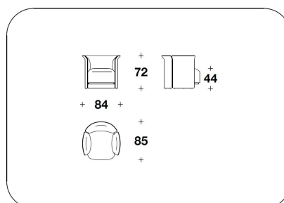
FET (POLE) VENEERED : POLTRONA / ARMCHAIR 84x85x72H. - H.S.44cm 33x33 1/3x28 1/3H. - H.S.17 1/4"
