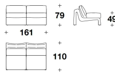
ING (E2) ELEMENTO 2 POSTI / 2 SEATER ELEMENT 161x110x79H. - H.S.49cm 63 1/3x43 1/3x31H. - H.S.19 1/4"
