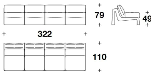
ING (E4) ELEMENTO 4 POSTI / 4 SEATER ELEMENT 322x110x79H. - H.S.49cm 126 2/3x43 1/3x31H. - H.S.19 1/4"
