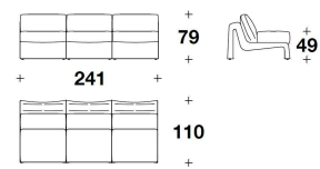
ING (E3) ELEMENTO 3 POSTI / 3 SEATER ELEMENT 241x110x79H. - H.S.49cm 95x43 1/3x31H. - H.S.19 1/4"
