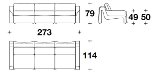
ING (D3) DIVANO 3 POSTI / 3 SEATER SOFA 273x114x79H. - H.S.49cm 107 1/3x45x31H. - H.S.19 1/4"
